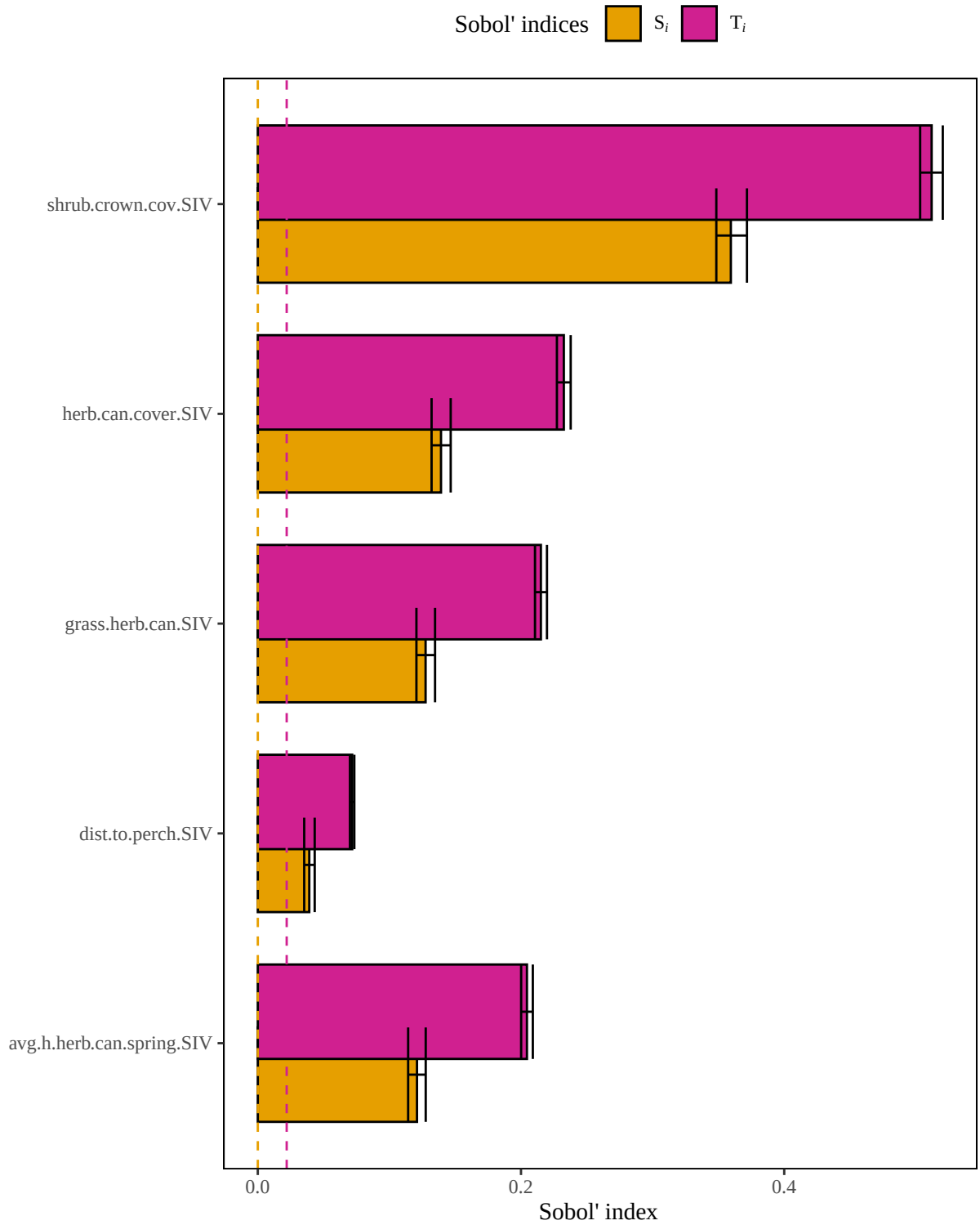
Figure 3. Results of a sensitivity analysis for the easternmeadowlark model based on the original author-specified model outlined in Schroeder and Sousa (1982). Dashed lines represent baseline numerical approximation error for S_i and T_i ( i.e. , dummy variables).
