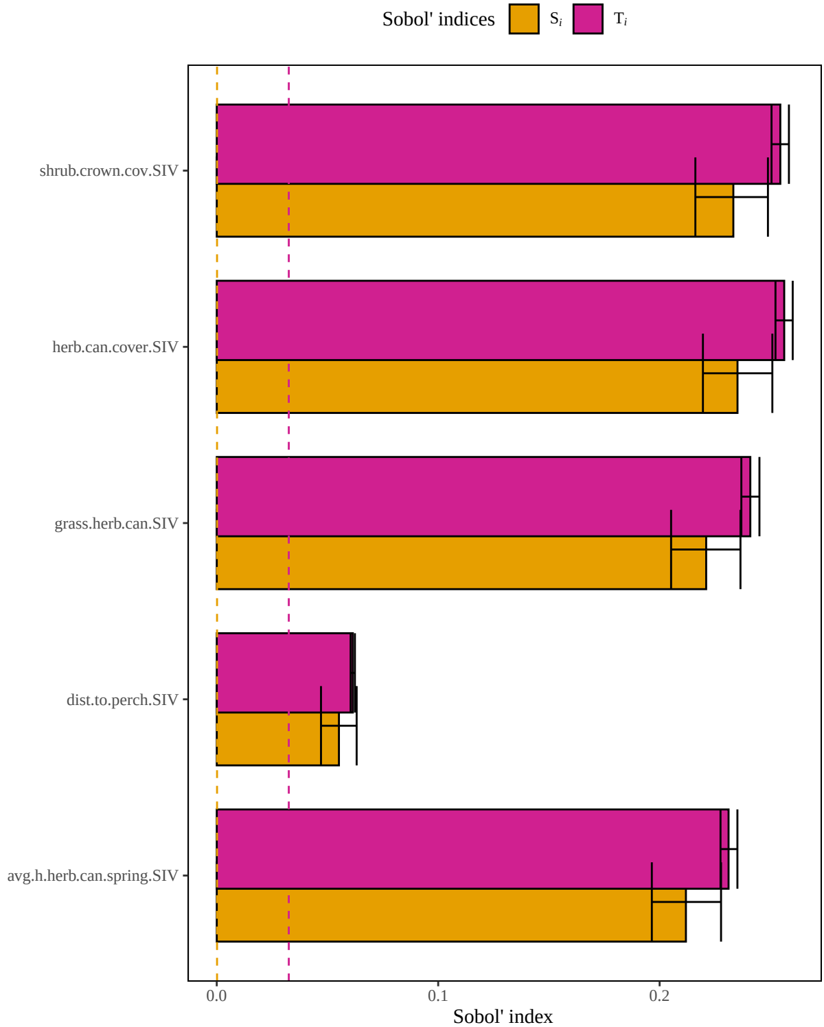
Figure 5. Results of a sensitivity analysis for the easternmeadowlark model based on a geometric mean structure. Dashed lines represent baseline numerical approximation error for S_i and T_i ( i.e. , dummy variables).
